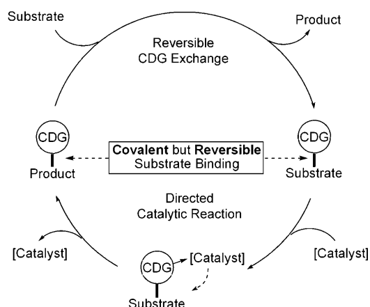
Figure 1. The concept of a catalyst-directing group (CDG) needed only in catalytic amounts through reversible covalent substrate binding.
