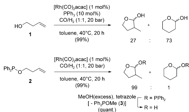
Scheme 1. Hydroformylation of homoallylic alcohol 1 with and without a covalently bound catalyst-directing phosphinite group ( 2 ). acac = acetylacetonate.
