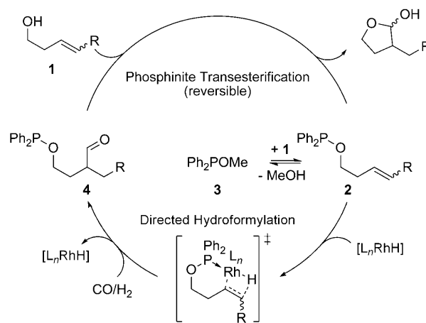
Figure 2. Proposed reaction scheme.
